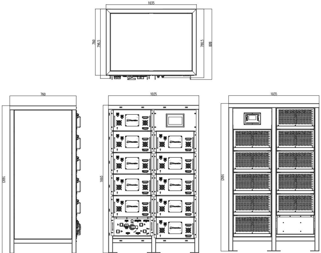
Figure Product dimension
