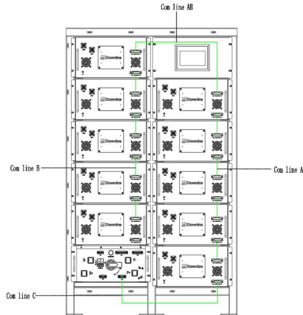
Figure Schematic diagram of battery cluster communication cable installation
