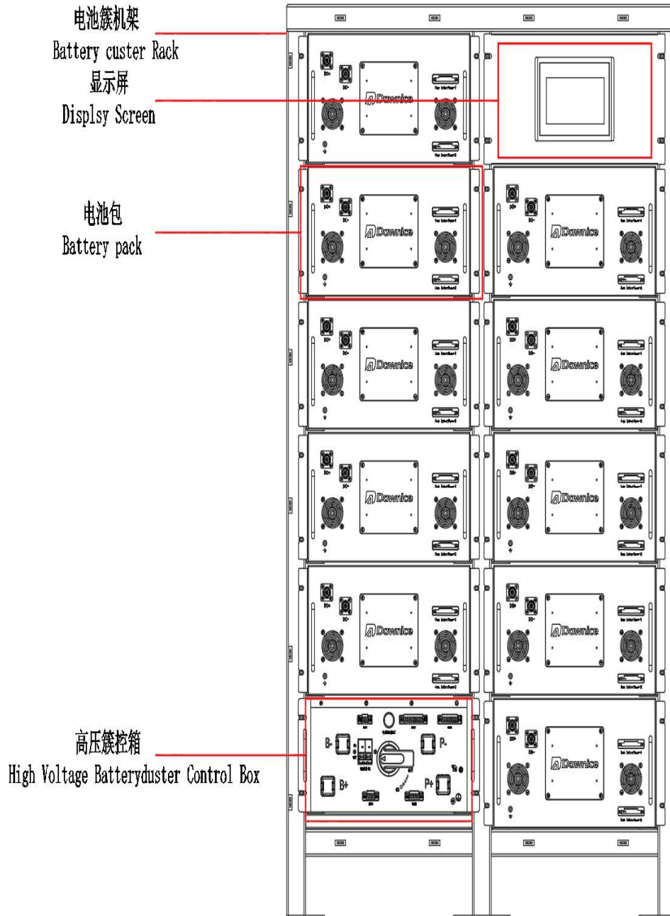
Figure Product layout-external
