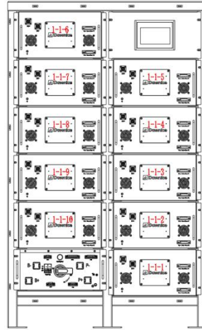
Figure 1. Battery pack installation sequence diagram
