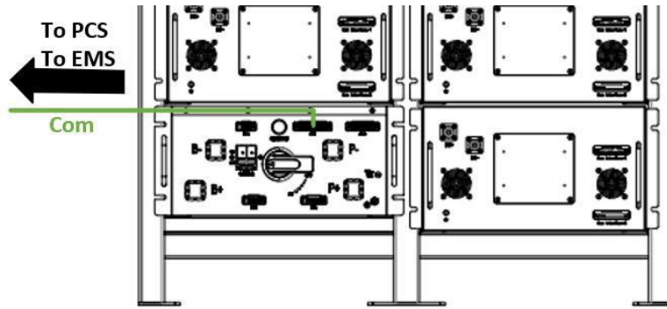
Figure Schematic diagram of battery cluster external communication cable installation
