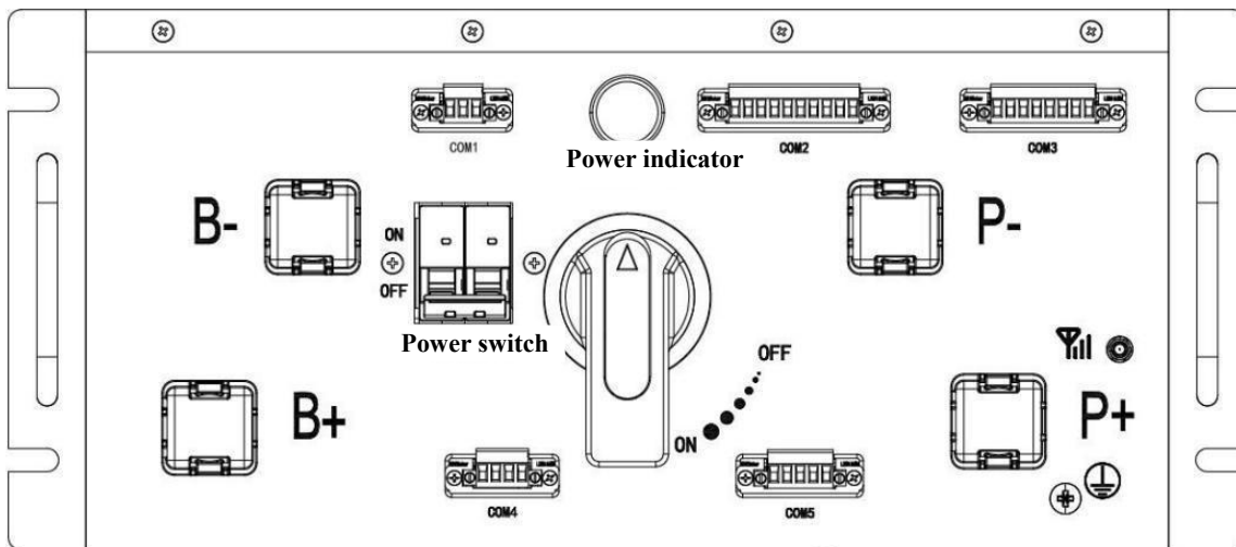
Figure Panel of high-voltage cluster control box
