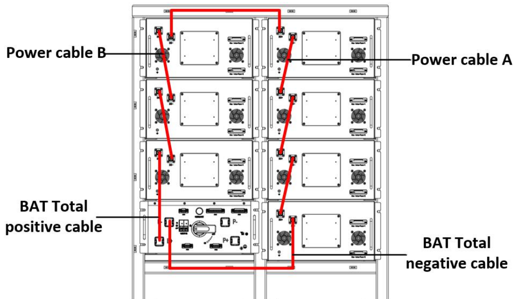
Figure Schematic diagram of battery cluster electrical cable installation
