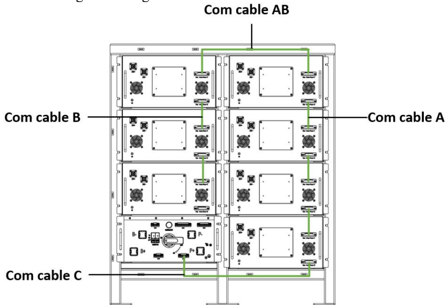
Figure Schematic diagram of battery cluster communication cable installation
