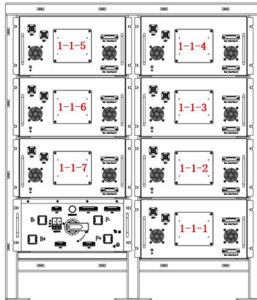
Figure 1. Battery pack installation sequence diagram
