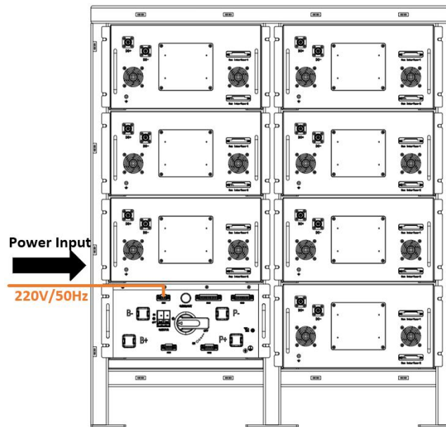
Figure Schematic diagram of battery cluster external power supply cable installation
