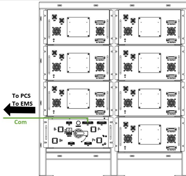
Figure Schematic diagram of battery cluster external communication cable installation
