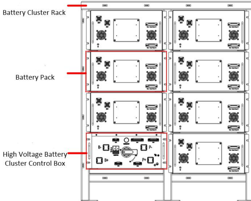
Figure Product layout-external
