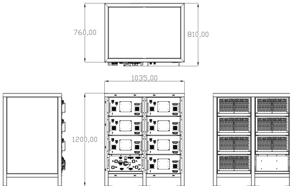
Figure Product dimension
