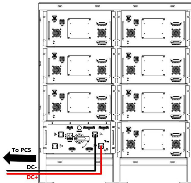
Figure Schematic diagram of battery cluster external electrical cable installation
