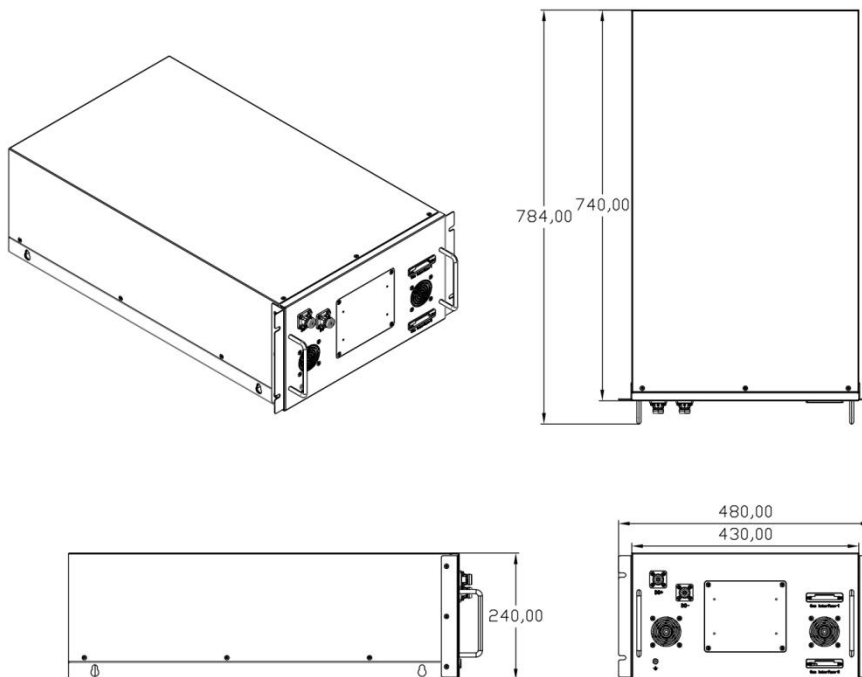
Figure 3-view of battery pack dimensions
