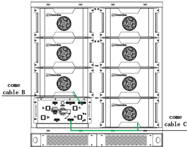
Battery cluster communication cable installation diagram
