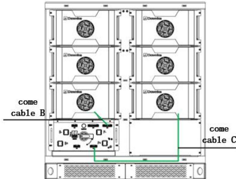
Battery cluster communication cable installation diagram
