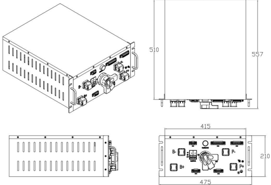
Figure Dimension of high-voltage cluster control box
