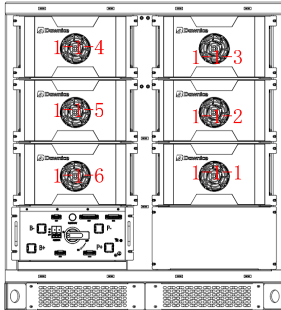
Figure 1. Battery pack installation sequence diagram
