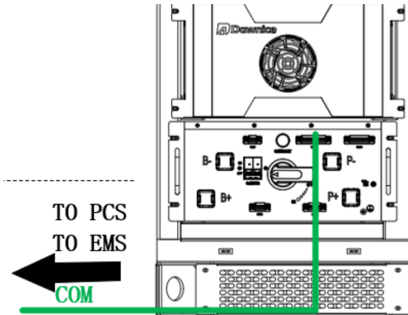
Figure Schematic diagram of battery cluster external electrical cable installation
