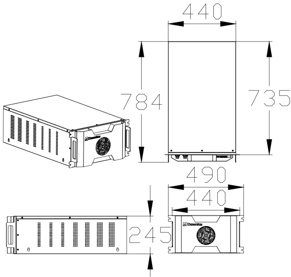
Figure 3-view of battery pack dimensions
