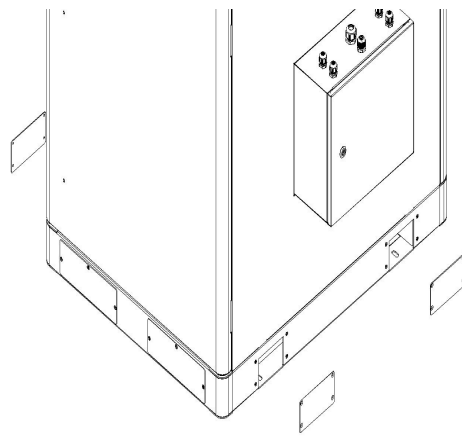
Figure-Diagram of disassembly and assembly of bottom baffle
