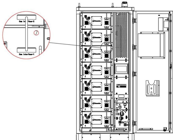
Figure-Diagram for disassembly and assembly of battery pack panel
