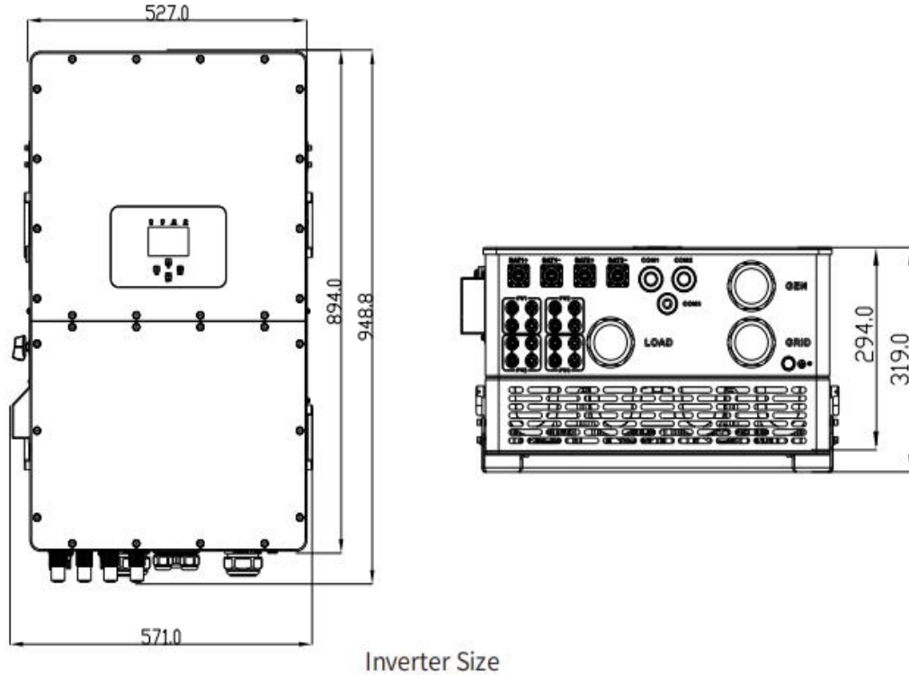
Figure Dimensions of the Converter
