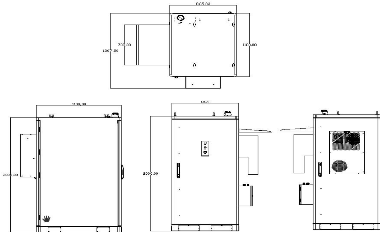
Figure Product dimension
