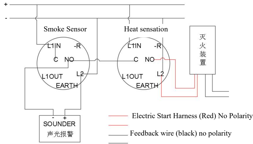
Figure Working principle of fire protection system
