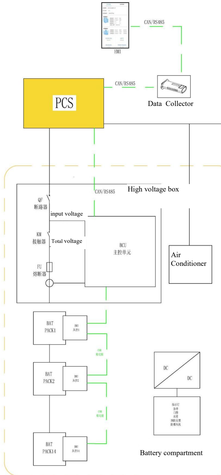
Figure Battery cabinet topology
