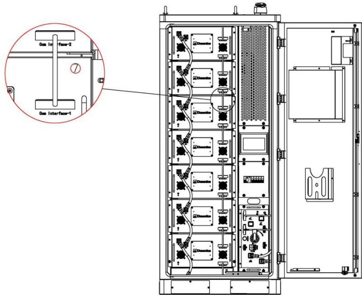
Figure-Installation diagram of battery pack connecting line
