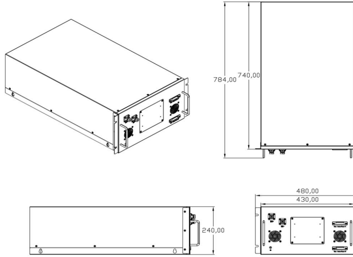
Figure Dimension of battery pack
